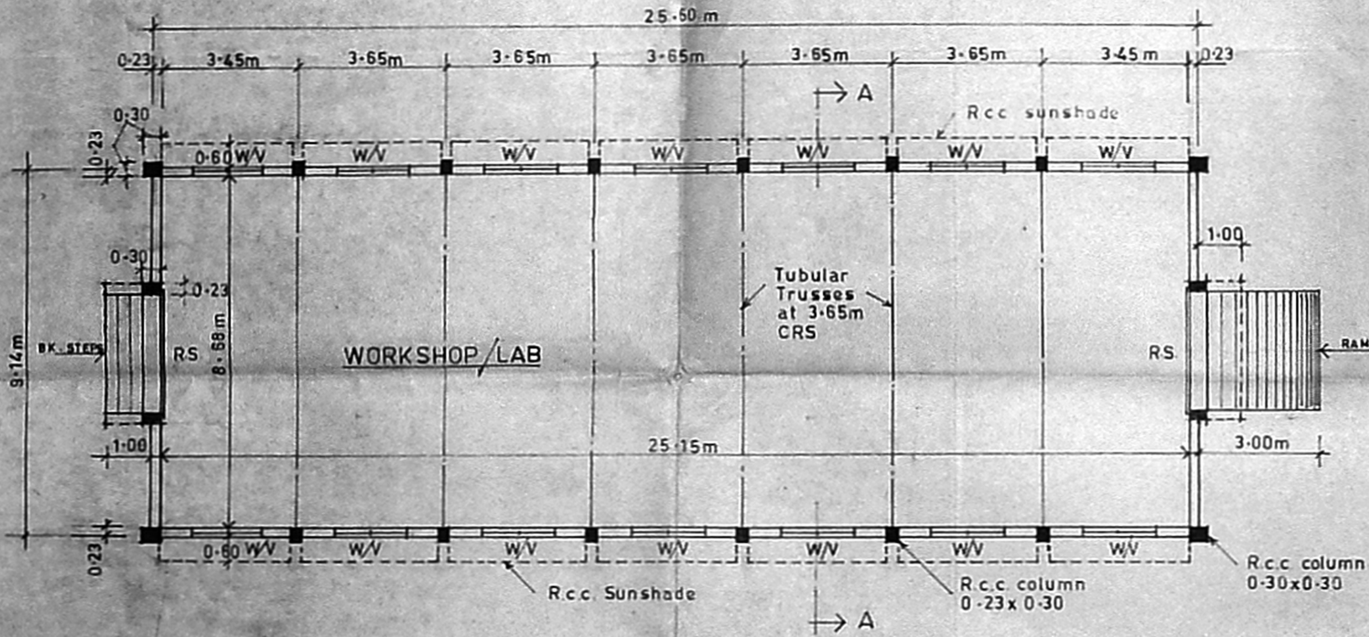
PLAN
