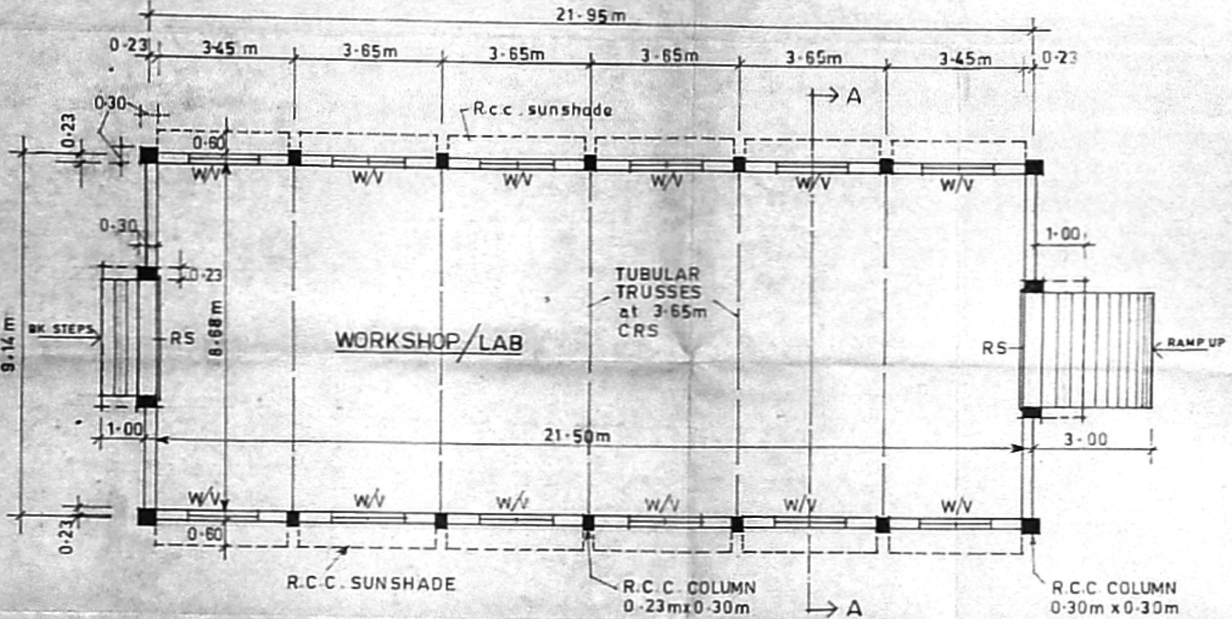
PLAN
