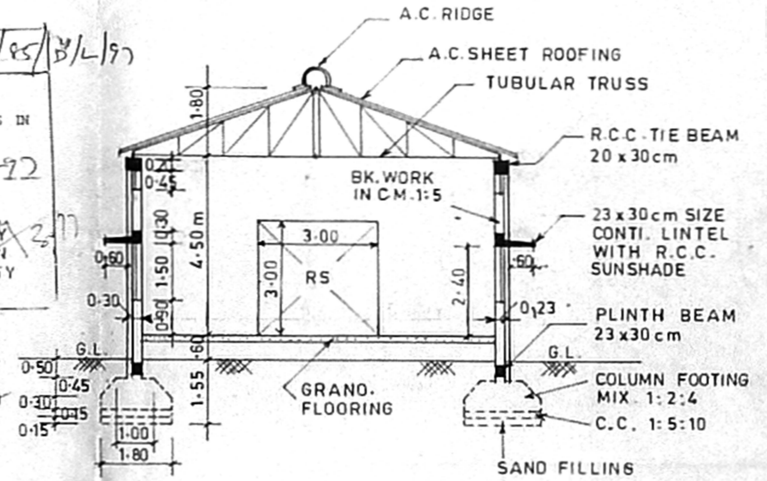
CROSS SECTION ON A/A
