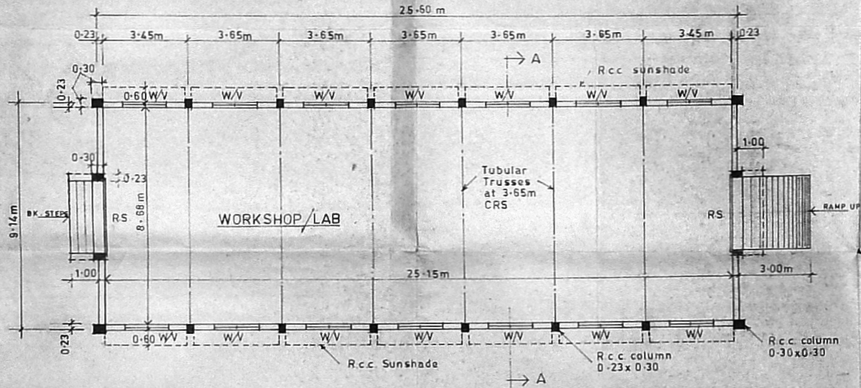
PLAN All Dimensions are in Metres
