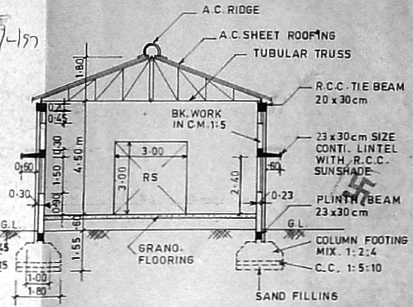
CROSS SECTION ON A/A
