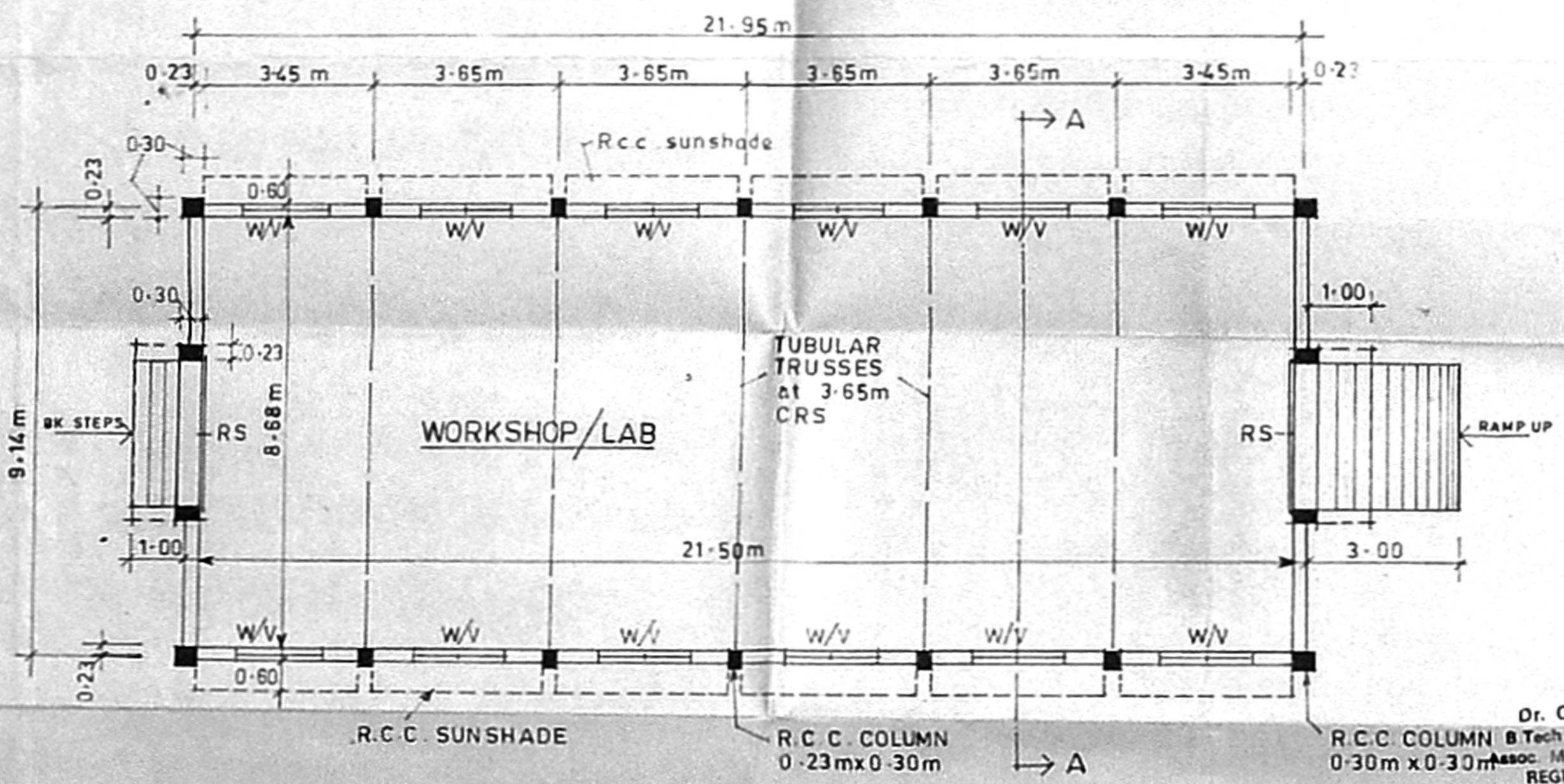
PLAN
