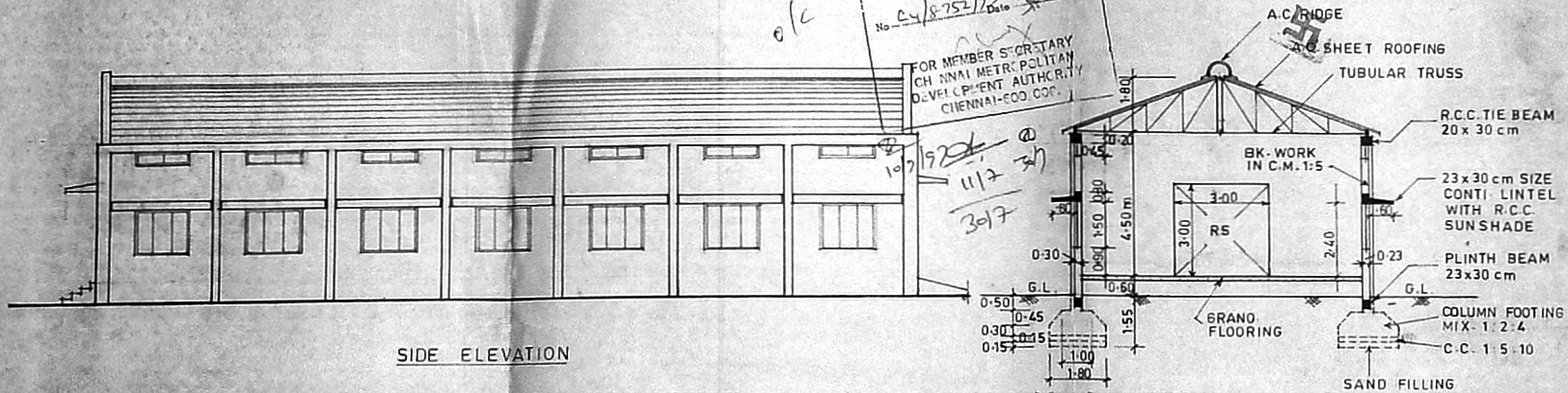
CROSS SECTION ON A/A
