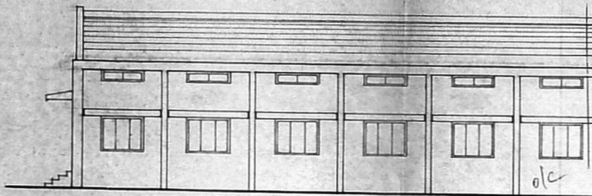
SIDE ELEVATION
