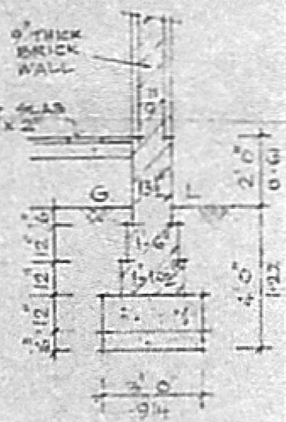
FOUNDATION DETAILS FOR 9" THICK BRICK GABLE WALL
